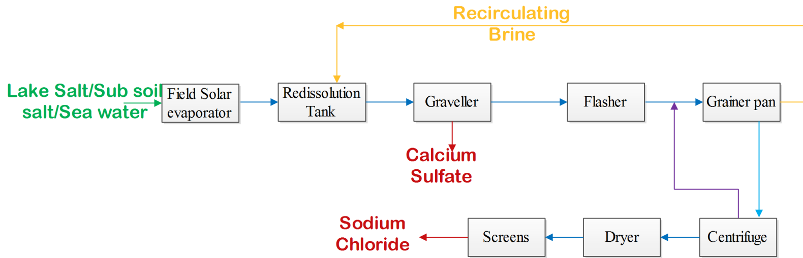
Figure: Manufacturing of Sodium Chloride by Solar Evaporation
